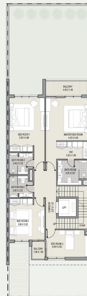
1ST FLOOR
