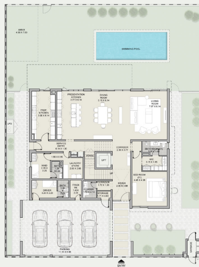
GROUND
