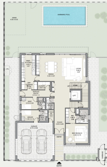
GROUND
