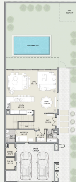
GROUND
